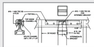
Intermediate Bracket
