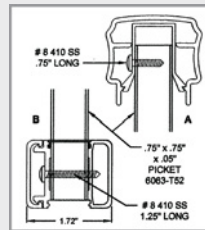
Intermediate Bracket
