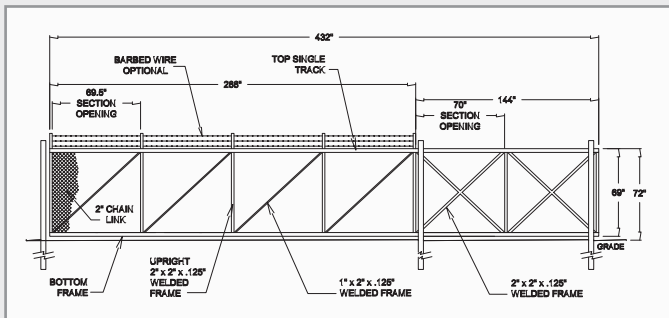
Chain Link Cantilever Gate (Detailed Example)
